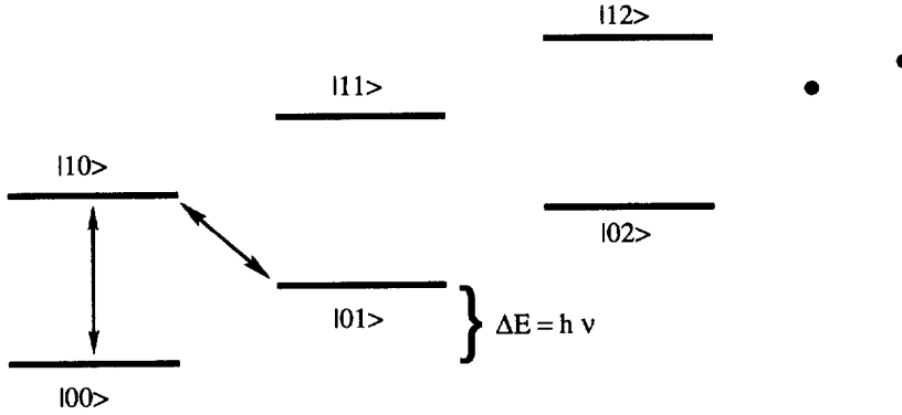
Fig. 12. The vertical axis gives the energy while the horizontal axis gives the degree of excitation of the center-of-mass mode. In |xy\rangle the first number x denotes the internal degree of freedom of the ion, while the second number y denotes the degree of excitation of the center-of-mass mode.
