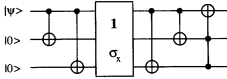
Fig. 14. The quantum network implementing an amplitude error correcting code. The initial state |\psi\rangle is encoded into three bits using two CNOT gates. If at most one bit-flip error occurs, indicated by the box, then the subsequent decoding and error correction using the TOFFOLI gate restores the state |\psi\rangle of the first qubit completely.
