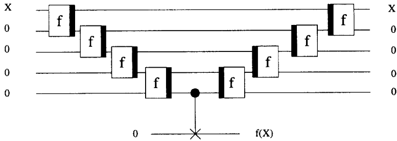
Fig. 8. How to get rid of garbage bits once the computation is performed. The network is the same in the classical and the quantum case, with the exception that quantum bits can, of course, be in an entangled state. Thick black bars on the left represent the reverse operation, i.e. the computation of f^{-1} .
