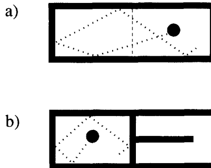
Fig. 3. (a) An atom-in-a-box representation of a bit: if the atom is in the left hand half of the box this represents a logical 0, whereas if it is in the right hand half this represents a logical 1; (b) confining the atom to one side, by pushing the piston, resets the bit to one of the two values thereby dissipating kT \ln 2 of heat.
