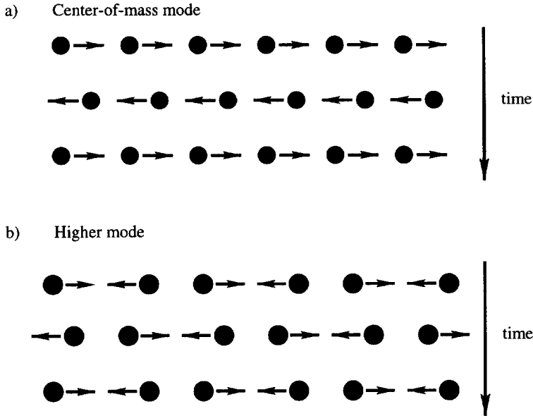
Fig. 11. In part (a) the center-of-mass mode is illustrated. All the ions oscillate with the same phase. In part (b) a mode of higher frequency is given. Here the ions have different phases and their relative distances change.
